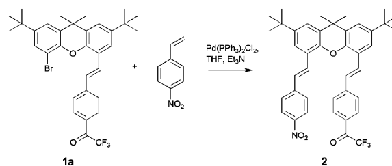
Scheme 2 Synthesis of compound 2.
