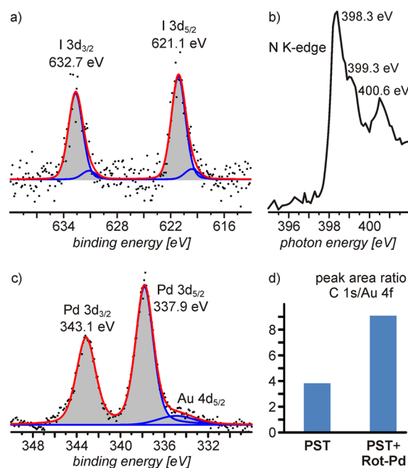
Figure 7. Deposition of Rot-Pd on a PST-SAM detected by (a) an I 3d doublet in the SR XP core level spectrum (in units of normalized (cps)) at 60° emission angle ( h\nu = 780 eV), (b) NEXAFS of the N K-edge (in units of normalized PEY (a.u.), 55°), (c) Pd 3d core level SR XP spectrum (in units of normalized (cps)) at 0° emission angle ( h\nu = 500 eV), and (d) peak area ratio C 1s/Au 4f (SR XPS, h\nu = 350 eV).
