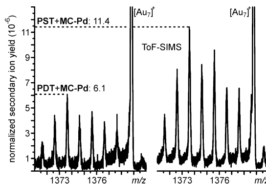
Figure 5. Comparison of the deposition of MC–Pd on a PDT- and PST–SAM expressed by normalized secondary ion yield ( 10^{-6} ) of [\text{MC} + \text{Pd}]^+ detected in the ToF-SIMS spectra.
