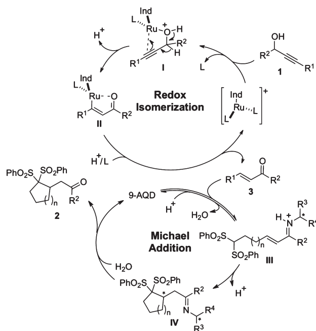
Scheme 4. Mechanistic Proposal for the Redox Cycloisomerization
