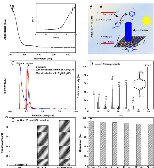
Fig. 4 UV-Vis diffusion reflectance spectrum of \text{Zn}_2\text{GeO}_4/\text{CFs} (the inset shows the relationship between (ah\nu)^2 and photon energy) (A), schematic illustration of photocatalytic oxidation mechanism of the p-toluidine over \text{Zn}_2\text{GeO}_4/\text{CFs} composites under UV-light irradiation (B), HPLC of p-toluidine solutions after UV irradiation over \text{Zn}_2\text{GeO}_4/\text{CFs} composites (C), the mass spectrum of product with RRT at 1.59 min (D), the percent conversions (PC) for oxidation of p-toluidine over CFs, pure \text{Zn}_2\text{GeO}_4 and \text{Zn}_2\text{GeO}_4/\text{CFs} tested under the same conditions (E) and reusability of \text{Zn}_2\text{GeO}_4/\text{CFs} for oxidation of p-toluidine (F).
