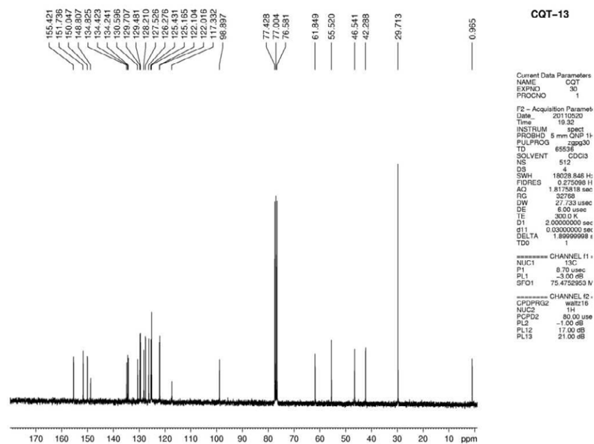
1 H and 13 C Spectrum of compound 12
