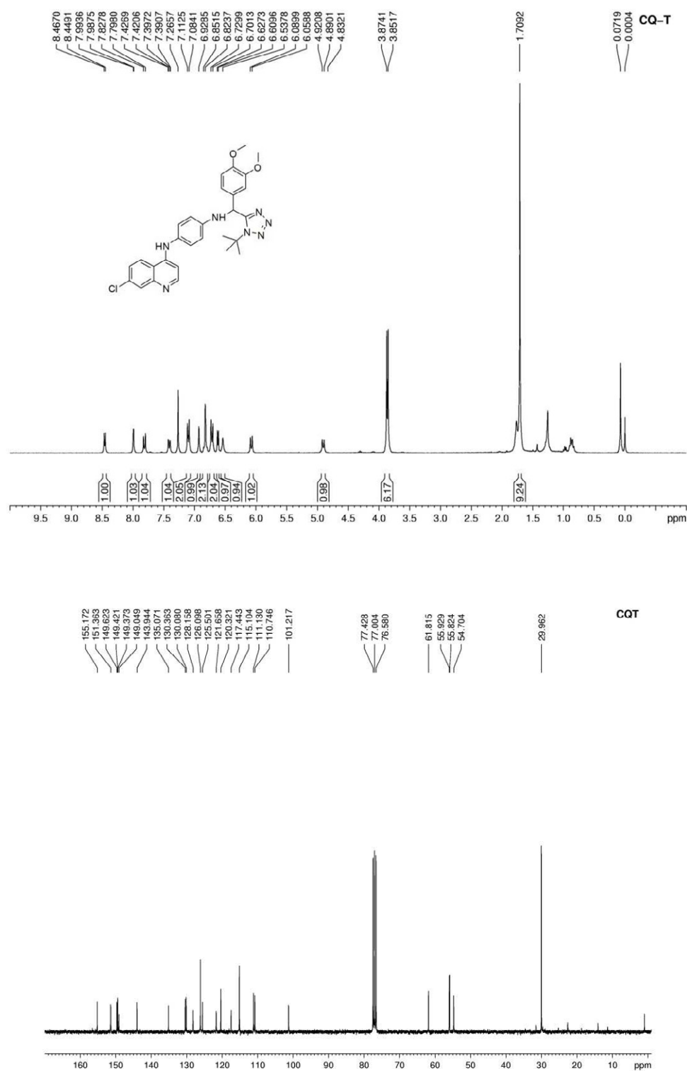
^1\text{H} and ^{13}\text{C} Spectrum of compound 18
