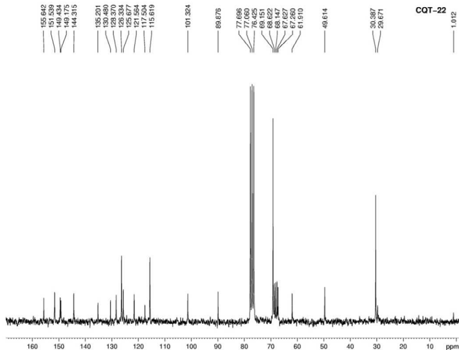
1 H and 13 C Spectrum of compound 31
