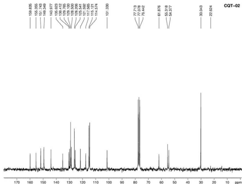
1 H and 13 C Spectrum of compound 17
