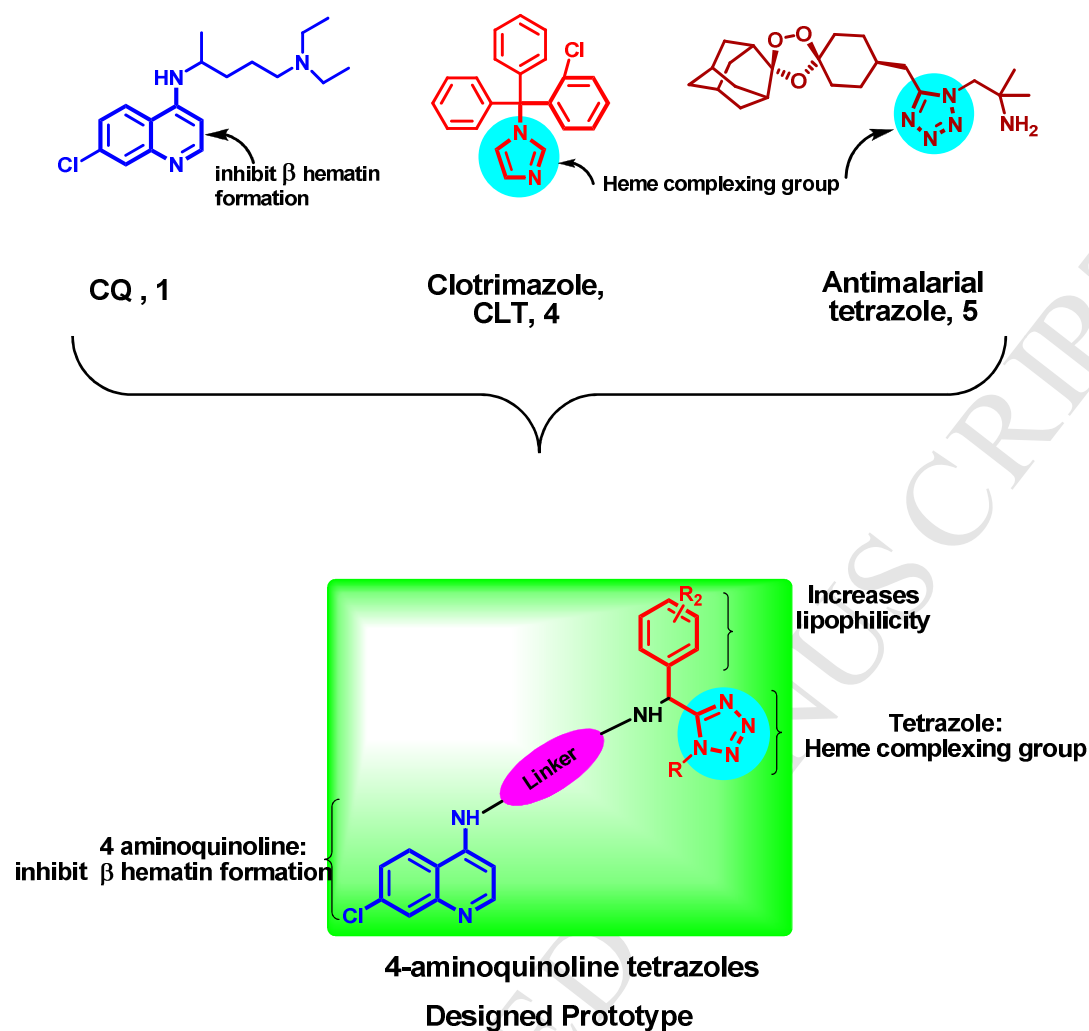
Figure 2: Basis for the synthesis of tetrazole derivatives of 4-aminoquinoline
