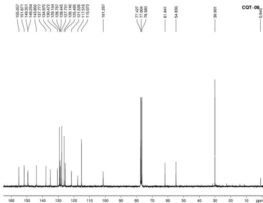
1 H and 13 C Spectrum of compound 24
