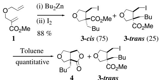
Scheme 2. Reagents and conditions: (i) Bu 2 Zn (3 equiv), Et 2 O, rt, 16 h; (ii) I 2 , THF, rt, 3 h.
