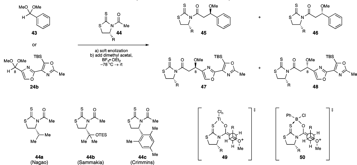
SCHEME 9. Condensation Reactions of N -Acetylthiazolidinethiones with Dimethyl Acetals
