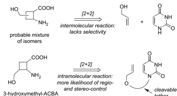
Figure 1. Retrosynthetic analysis.
