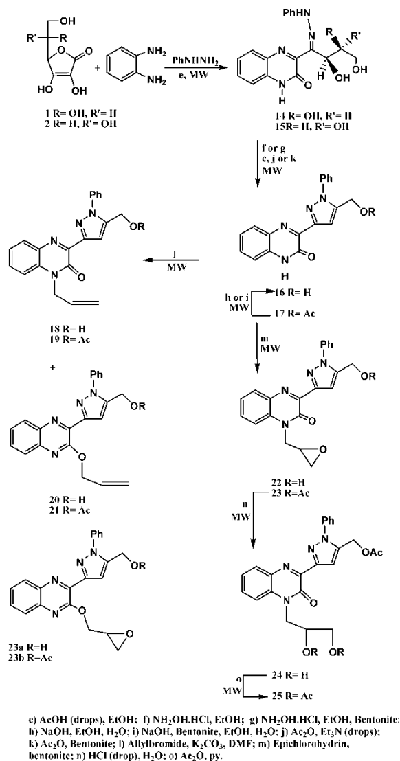
Scheme 2: Alkylation of quinoxalinone.
