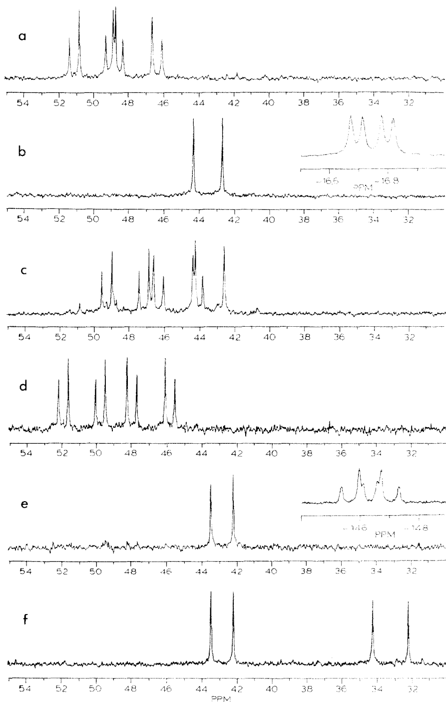
Fig. 1. a. ^{31}\text{P}\{^1\text{H}\} spectrum of Ia, \text{L} = \text{py} ; b. ^{31}\text{P}\{^1\text{H}\} and high field ^1\text{H} spectra of III, \text{L} = \text{py} ; c. ^{31}\text{P}\{^1\text{H}\} spectrum showing signals from Ib, \text{L}' = 2,6\text{-Me}_2\text{py} and III, \text{L} = \text{py} ; d. ^{31}\text{P}\{^1\text{H}\} spectrum of Ia, \text{L} = \text{N-Melm} ; e. ^{31}\text{P}\{^1\text{H}\} and high field ^1\text{H} spectra of IV, \text{L} = \text{N-Melm} ; f. ^{31}\text{P}\{^1\text{H}\} spectrum showing signals from IV, \text{L} = \text{N-Melm} and V, \text{L}' = 2,6\text{-Me}_2\text{py} .
