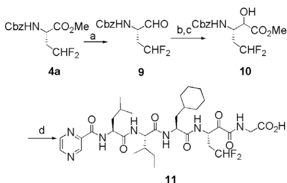
Scheme 3. Reagents and conditions: (a) DiBAL, CH 2 Cl 2 , -78^{\circ}\text{C} , 30 min (89%); (b) LiC(SMe) 3 , THF, -64^{\circ}\text{C} to -30^{\circ}\text{C} , 1 h (85%); (c) HgCl 2 /HgO, MeOH/H 2 O, rt, 2 h (96%); (d) Ref. 2.
