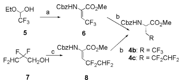
Scheme 2. Reagents and conditions: (a) KO t Bu, THF, -78^{\circ}\text{C} to rt (78%); (b) H 2 , 55 psi, [( S,S )-Et-Duphos-Rh] + CF 3 SO 3 − , MeOH (>95%), (i) Dess–Martin, DCM, rt, (ii) KO t Bu, THF, -78^{\circ}\text{C} to rt (38%).
