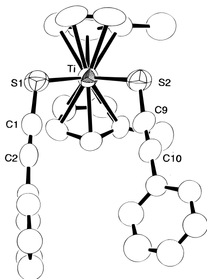
Figure 1. Structure of \text{MeCp}_2\text{Ti}(\text{SC}\equiv\text{CPh})_2 ( 4 ).
