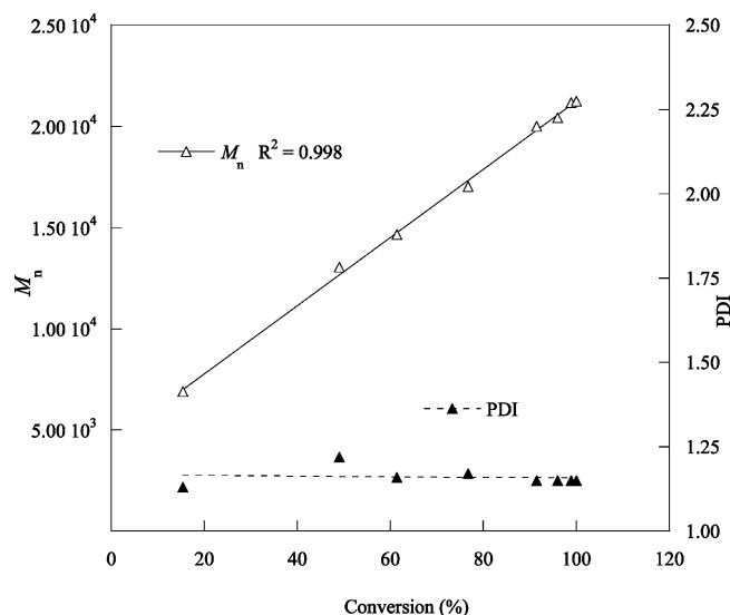
Figure 6. Plots of M_n and PDI of PMMA vs MMA conversion in toluene at 25 °C: [MMA]_0 = 0.935 M, [6]_0 = [Ph_3C][B(C_6F_5)_4]_0 = 4.67 mM with a [MMA]_0/[catalyst]_0 ratio of 200/1.
