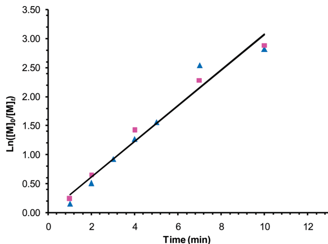
Figure 5. Plots of the first-order kinetics of \ln([MMA]_0/[MMA]_t) vs time (min) for the polymerization of MMA by 6 (pink ■) and 10 (blue ▲) activated with equimolar [Ph_3C][B(C_6F_5)_4] in toluene at 25 °C. Conditions: [MMA]_0 = 0.935 M, [Zr]_0 = 2.34 mM.
