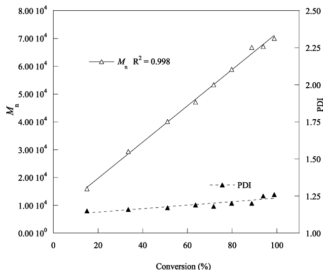
Figure 7. Plots of M_n and PDI of PMMA vs MMA conversion in toluene at 25 °C: [MMA]_0 = 0.935 M, [6]_0 = [Ph_3C][B(C_6F_5)_4]_0 = 0.935 mM with a [MMA]_0/[catalyst]_0 ratio of 1000/1.
