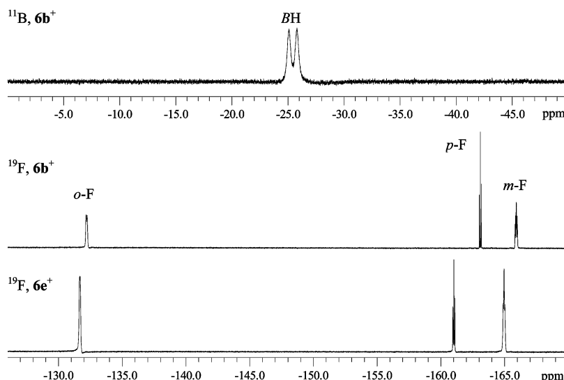
Figure 4. ^{11}\text{B} NMR ( \text{CD}_2\text{Cl}_2 ) (top, 23 °C) and ^{19}\text{F} NMR (middle, 23 °C) spectra of 6\text{b}^+[\text{HB}(\text{C}_6\text{F}_5)_3]^- (top, 23 °C) and ^{19}\text{F} NMR ( \text{CD}_2\text{Cl}_2 ) spectrum of 6\text{e}^+[\text{B}(\text{C}_6\text{F}_5)_4]^- (bottom, -60 °C).
