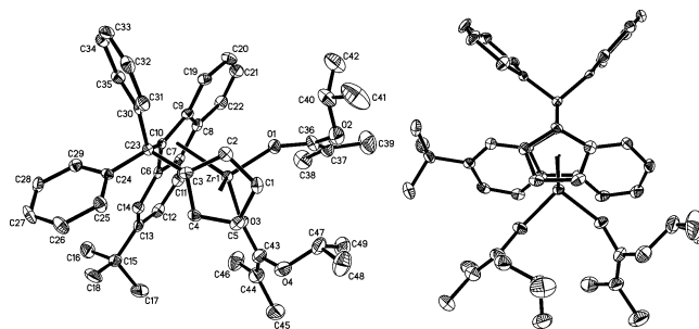
Figure 1. Molecular structure of [Ph 2 C(Cp)(2'-Bu-Flu)]Zr[OC(O i Pr)=CMe 2 ] 2 ( 7 ) with thermal ellipsoids drawn at the 50% probability. Selected bond lengths (Å): Zr–O(1) = 1.964(3), Zr–O(3) = 1.981(3), Zr–C(1) = 2.546(4), Zr–C(2) = 2.491(4), Zr–C(3) = 2.490(4), Zr–C(4) = 2.486(4), Zr–C(5) = 2.539(4), Zr–C(6) = 2.575(4), Zr–C(9) = 2.571(4), Zr–C(10) = 2.491(4), Zr–C(7) = 2.735(4), Zr–C(8) = 2.727(4).
