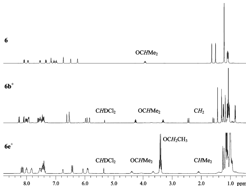
Figure 3. ^1\text{H} NMR spectra of precatalyst 6 (top, \text{C}_6\text{D}_6 , 23 °C) as well as cationic ester enolate catalysts 6\text{b}^+[\text{HB}(\text{C}_6\text{F}_5)_3]^- (middle, \text{CD}_2\text{Cl}_2 , 23 °C) and 6\text{e}^+[\text{B}(\text{C}_6\text{F}_5)_4]^- (bottom, \text{CD}_2\text{Cl}_2 , -60 °C). Only the most diagnostic peaks are assigned here (see Experimental Section for complete assignments).
