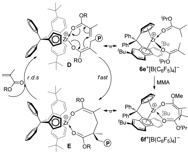
Scheme 4. Proposed Mechanism of Methacrylate Polymerization Catalyzed by 6^+[B(C_6F_5)_4]^-
