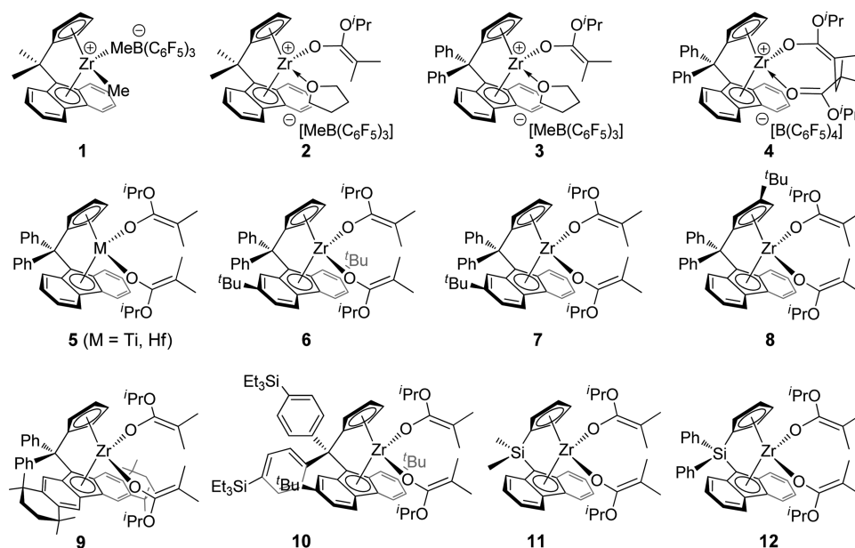
Chart 1. Ansa-Zirconocene Complexes Incorporating C_5 -Symmetric [R_2E(Cp)(Flu)] -Based Ligands and Their Variants Investigated in This Study
