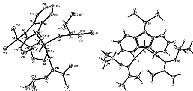
Figure 2. Molecular structure of [Me 2 Si(Cp)(Flu)]Zr[OC(O i Pr)=CMe 2 ] 2 ( 11 ) with thermal ellipsoids drawn at the 50% probability. Selected bond lengths (Å): Zr–O(1) = 1.9923(8), Zr–O(3) = 1.9698(7), Zr–C(1) = 2.5308(10), Zr–C(2) = 2.5416(11), Zr–C(3) = 2.4922(11), Zr–C(4) = 2.5007(10), Zr–C(5) = 2.4874(10), Zr–C(7) = 2.6173(10), Zr–C(8) = 2.4975(10), Zr–C(9) = 2.6117(10), Zr–C(6) = 2.7378(10), Zr–C(10) = 2.7611(10), Zr–Cp(centroid) = 2.201, Zr–Flu(centroid) = 2.345.
