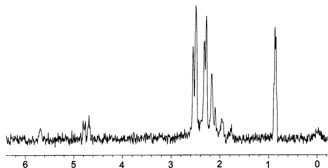
Figure 15. ^2\text{H} NMR spectrum of neat 3,3-dimethylbutene with 0.5 mol % of complex 8 , after 4 h at 35 ^{\circ}\text{C} .
