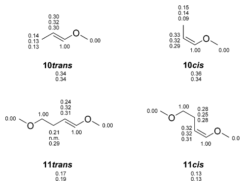
Figure 17. Molar fractions of compounds 10cis , 10trans , 11cis , and 11trans in the product (under the compound number) and molar fractions of deuteration at each position. The number on top was based on the proton spectrum and the second number on the deuterium spectrum. The number on the bottom for the molar fraction of deuteration was based on the integral of the proton signal at that position and the composition determined in the deuterium spectrum, and it is the most reliable.
