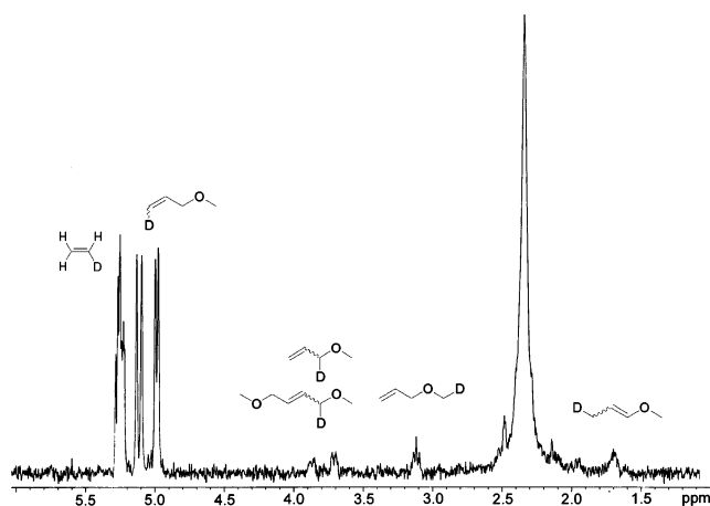
Figure 14. ^2\text{H} NMR spectrum of neat allyl methyl ether with 0.5 mol % of complex 8 , after 4 h at 35 ^{\circ}\text{C} .
