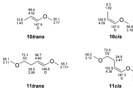
Figure 16. ^1\text{H} and ^{13}\text{C} chemical shift assignments in the compounds 10cis , 10trans , 11cis , and 11trans .
