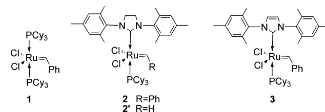
Figure 1. Olefin metathesis catalysts.
