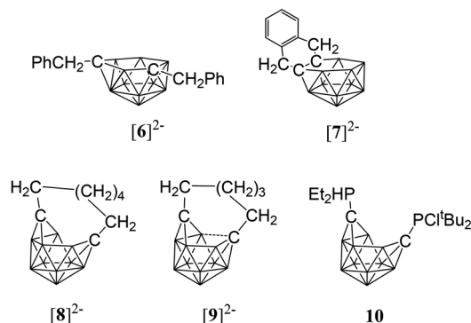
Fig. 11 Geometries of nido -dicarbadodecaboranes determined by X-ray crystallography.
