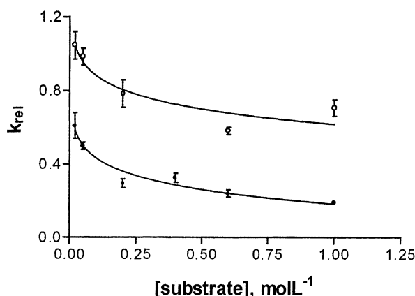
Figure 3. Variation of the relative rate for (○) vinyl butyl ether ( k_e/k_o ) and (●) vinyl butyrate ( k_{\text{es}}/k_o ) with the concentration of the substrate.
