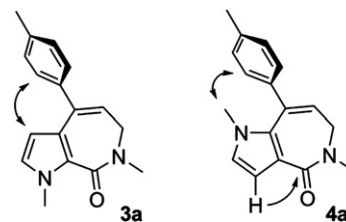
Figure 2. Relevant NOE (double arrows) and HMBC (single arrow) correlations of compounds 3a and 4a .
