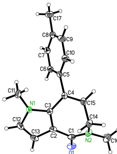
Figure 3. ORTEP view of the molecular structure of 1,5-dimethyl-8- p -tolyl-5,6-dihydro-1 H -pyrrolo[3,2- c ]azepin-4-one ( 4a ). The thermal ellipsoids correspond to 30% probability.
