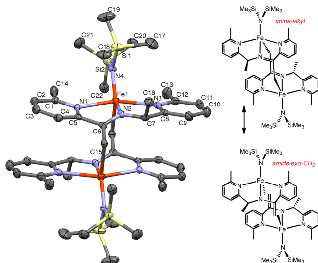
Figure 7. Molecular view of [\{(\text{Me}_3\text{Si})_2\text{N}\}\text{Fe}]_2(\mu\text{-}\kappa^4, \kappa^4\text{-N,py}_2, \text{C-}(^b\text{Me}, ^b\text{CH}_2, ^o\text{Me}_2(\text{smif})\text{H}))_2 ( 9 ) and plausible valence bond structures. Selected interatomic distances (Å) and angles (deg): Fe–Fe, 4.7420(5); Fe–N1, 2.3192(17); Fe–N2, 2.0511(15); Fe–N3, 2.3538(17); Fe–N4, 1.9914(16); Fe–C15', 2.336(2); Fe–C6', 2.889(2); N2–C6, 1.331(2); N2–C7, 1.465(3); C6–C15, 1.375(3); N1–Fe–N2, 75.18(6) ; N1–Fe–N3, 149.14(6) ; N1–Fe–N4, 102.19(6) ; N2–Fe–N3, 74.29(6) ; N2–Fe–N4, 136.76(7) ; N3–Fe–N4, 102.96(6) ; N1–Fe–C15', 91.07(7) ; N2–Fe–C15', 106.59(7) ; N3–Fe–C15', 93.39(7) ; N4–Fe–C15', 116.64(7) .
