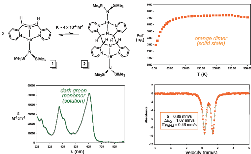
Figure 3. Green (\text{smif})\text{Fe}[\text{N}(\text{SiMe}_3)_2] ( 1 ) is monomeric in solution, but in the solid state, it is a dimer, [(\text{Me}_3\text{Si})_2\text{N}]\text{Fe}_2(\mu\text{-}\kappa^3\text{-N,py}_2\text{-smif,smif}) ( 2 , X-ray). A \mu_{\text{eff}} vs T (K) plot and a Mössbauer spectrum of 2 are shown.
