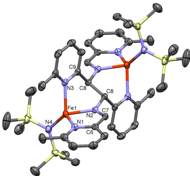
Figure 5. Molecular view of [\{(\text{Me}_3\text{Si})_2\text{N}\}\text{Fe}]_2(\mu:\kappa^3\text{-N,py,py}',\kappa^3\text{-N}',\text{py}',\text{-py-}^o\text{Me}_2\text{smif-}^o\text{Me}_2\text{smif}) ( 6 ). Selected interatomic distances ( \text{\AA} ) and angles ( ^\circ ): Fe-Fe, 5.941(2) ; Fe-N1, 2.0965(15) ; Fe-N2, 2.0069(15) ; Fe-N3, 2.1464(15) ; Fe-N4, 1.9489(15) ; N1-C6, 1.381(2) ; C6-C7, 1.405(3) ; N2-C7, 1.328(2) ; N2-C8, 1.448(2) ; C8-C8, 1.561(2) ; N1-Fe-N2, 79.19(6) ; N1-Fe-N3, 108.95(6) ; N1-Fe-N4, 118.19(7) ; N2-Fe-N3, 83.70(6) ; N2-Fe-N4, 129.78(6) ; N3-Fe-N4, 125.16(6) ; C7-N2-C8, 118.73(15) ; N2-C8-C8, 107.79(17) ; C8-C8-C9, 109.72(17) .
