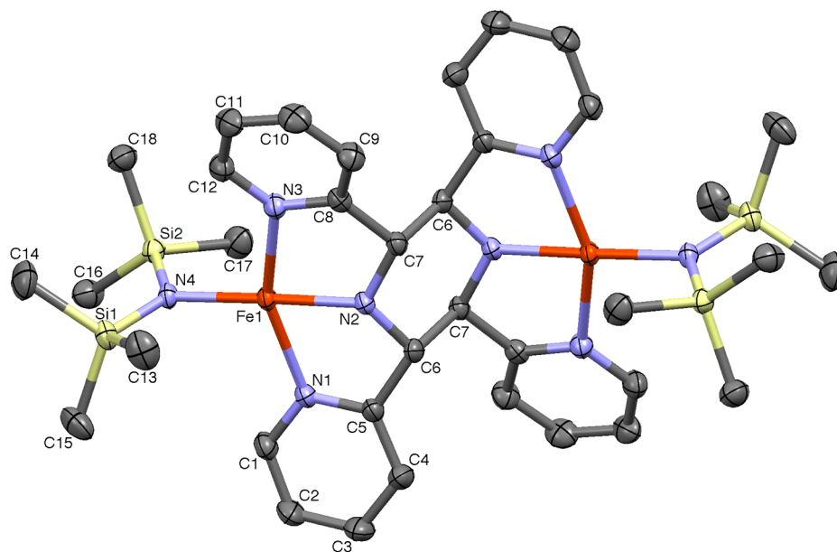
Figure 4. Molecular view of [(\text{Me}_3\text{Si})_2\text{N}\text{Fe}]_2(\mu\text{-}\kappa^3, \kappa^3\text{-N,py}_2\text{-smif,smif}) ( 2 ). Selected interatomic distances (Å) and angles (deg): Fe–Fe, 6.158(2); Fe–N1, 2.1950(11); Fe–N2, 1.9432(10); Fe–N3, 2.1910(11); Fe–N4, 1.9538(10); N2–C7, 1.4356(16); N2–C6, 1.4334(17); C7–C8, 1.4964(18); C5–C6, 1.5023(17); C6–C7, 1.5781(18); N4–Si1, 1.6983(11); N4–Si2, 1.6966(11); N1–Fe–N2, 77.20(4); N1–Fe–N3, 154.48(4); N1–Fe–N4, 101.94(4); N2–Fe–N3, 77.38(4); N2–Fe–N4, 178.53(4); N3–Fe–N4, 103.43(4); Fe–N2–C6, 120.95(8); Fe–N2–C7, 120.66(8); C6–Fe–C7, 113.94(10); N2–C6–C5, 108.09(10); N2–C6–C7, 109.08(10); N2–C7–C6, 108.93(10); N2–C7–C8, 108.03(10); C5–C6–C7, 112.72(10); C6–C7–C8, 113.10(11).
