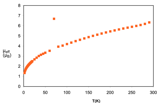
Figure 6. Plot of \mu_{\text{eff}} vs T (K) for dimer [\{(\text{Me}_3\text{Si})_2\text{N}\}\text{Fe}]_2(\mu\text{-}\kappa^4, \kappa^4\text{-N,py}_2, \text{C-}(^b\text{Me}, ^b\text{CH}_2, ^o\text{Me}_2(\text{smif})\text{H}))_2 ( 9 ).
