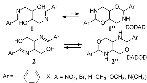
Scheme 1. The 1,4-bis(arylideneamino)-2,3-butanediol ( 1 )/dioxadiazadecalin (DODAD, 1'' ) and 2,3-bis(arylideneamino)-1,4-butanediol ( 2 )/diazadioxadecalin (DADOD, 2'' ) equilibria.
