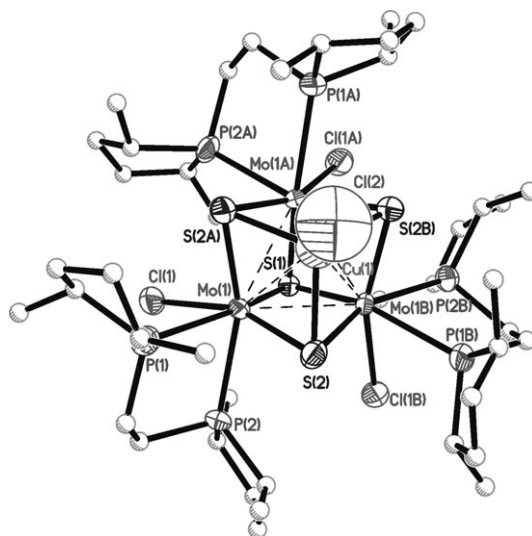
Figure 3. ORTEP plot of [Mo 3 CuS 4 {(S,S)-Me-BPE} 3 Cl 4 ]CuCl 2 [(M)-2]CuCl 2 with the atom-numbering scheme (50 % probability ellipsoids). Carbon atoms are drawn as spheres for clarity. Selected bond lengths [Å]: Mo–Mo 2.804(2), Mo(1)–(μ 3 -S(1)) 2.352(6), Mo(1)–(μ 3 -S(2)) 2.311(5), Mo(1)–(μ 3 -S(2A)) 2.368(5), Mo(1)–P(1) 2.590(5), Mo(1)–P(2) 2.632(5), Mo(1)–Cl 2.458(5), Mo(1)–Cu(1) 2.843(3), Cu(1)–(μ 3 -S(2)) 2.312(5), Cu(1)–Cl 2.18(1).
