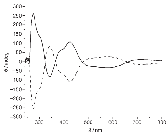
Figure 4. Circular dichroism spectra of [\text{Mo}_3\text{CuS}_4\{(\text{R,R})\text{-Me-BPE}\}_3\text{Cl}_4]\text{-CuCl}_2 ( [(\text{P})\text{-2}]^+ , —) and [\text{Mo}_3\text{CuS}_4\{(\text{S,S})\text{-Me-BPE}\}_3\text{Cl}_4]\text{-CuCl}_2 ( [(\text{M})\text{-2}]^+ , ---) in dichloromethane ( 1.33 \times 10^{-4} and 1.35 \times 10^{-4} M, respectively) at 25°C.
