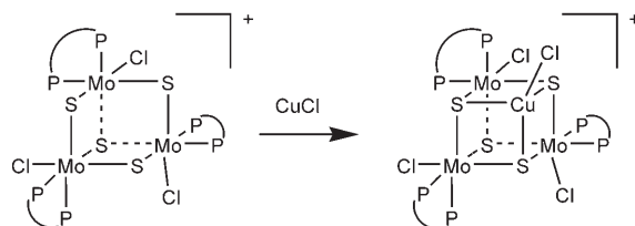
Scheme 1. General synthetic procedure for [\text{Mo}_3\text{Cu}(\text{diphosphane})_3\text{Cl}_4]^+ clusters.
