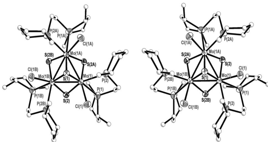
Figure 2. ORTEP plot of [Mo 3 S 4 {(R,R)-Me-BPE} 3 Cl 3 ]PF 6 [(P)-1]PF 6 , (left) and [Mo 3 S 4 {(S,S)-Me-BPE} 3 Cl 3 ]PF 6 [(M)-1]PF 6 , (right) with the atom-numbering scheme (50 % probability ellipsoids). Carbon atoms are drawn as spheres for clarity. Selected bond lengths [Å]: [(P)-1]PF 6 : Mo–Mo 2.8011(8), Mo(1)–(μ 3 -S(1)) 2.360(2), Mo(1)–(μ 3 -S(2)) 2.327(2), Mo(1)–(μ 3 -S(2A)) 2.283(2), Mo(1)–P(1) 2.568(2), Mo(1)–P(2) 2.641(2), Mo–Cl 2.487(2); [(M)-1]PF 6 : Mo–Mo 2.7975(9), Mo(1)–(μ 3 -S(1)) 2.362(2), Mo(1)–(μ 3 -S(2)) 2.322(2), Mo(1)–(μ 3 -S(2A)) 2.282(2), Mo(1)–P(1) 2.558(2), Mo(1)–P(2) 2.633(2), Mo–Cl 2.485(2).
