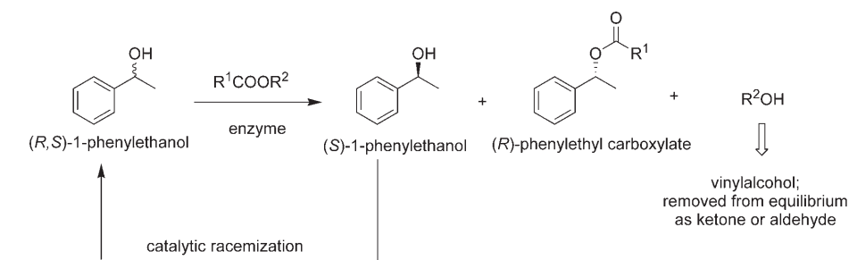
Scheme 1. Dynamic resolution of 1-phenylethanol.
