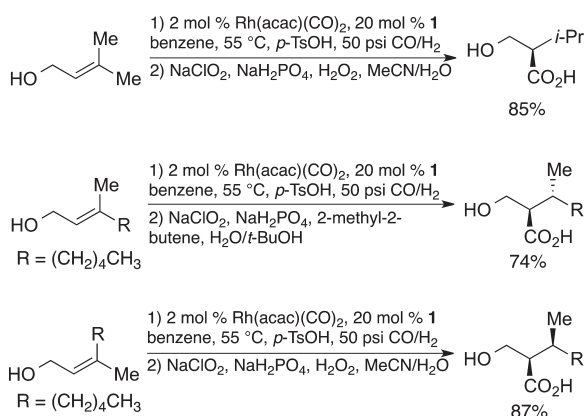
Scheme 1. Hydroformylation of Trisubstituted Olefins
