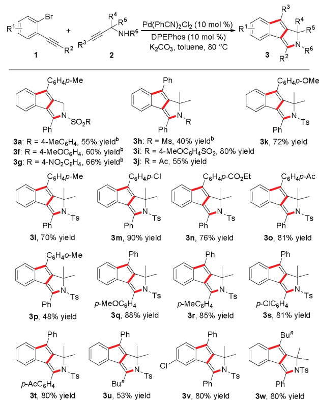
Scheme 3. Palladium-Catalyzed Tandem Reaction of 2-Alkynylbromobenzene 1 with Propargylic Sulfonamide 2 a
