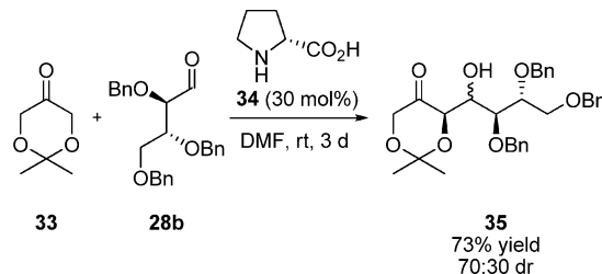
Scheme 8. Transformation of 28b into Protected Ketoheptose 35
