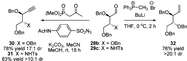
Scheme 7. Homologation of Aldehydes 28b and 29c
