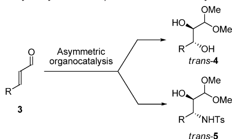
Scheme 3. Formal trans -Dihydroxylation and trans -Aminohydroxylation of \alpha,\beta -Unsaturated Aldehydes 3
