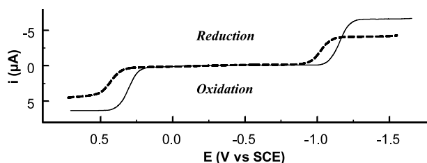
Fig. 3. RDE voltammogram of 4.1\text{ mM} [\text{Nb}(\eta^5\text{-C}_5\text{H}_4\text{SiMe}_3)_2\text{Cl}_2] ( 12a ) (plain line) and 3.7\text{ mM} [\text{Nb}\{\text{Me}_2\text{Si}(\eta^5\text{-C}_5\text{H}_3\text{SiMe}_3)\}_2\text{Cl}_2] ( 11a ) (dashed line) in THF 0.2\text{ M} \text{NBu}_4\text{PF}_6 . Sweep rate: 20\text{ mV s}^{-1} .
