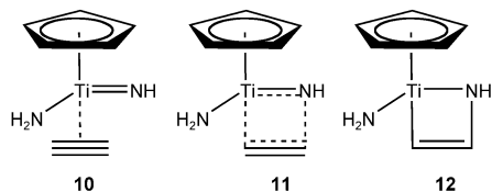
Scheme 5. [2+2]-Cycloaddition: 10 ( \pi -complex); 11 (transition state) and 12 (intermediate).
