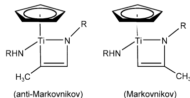
Scheme 6. [2+2]-Cycloaddition products with \text{CH}_3\text{C}\equiv\text{CH} .
