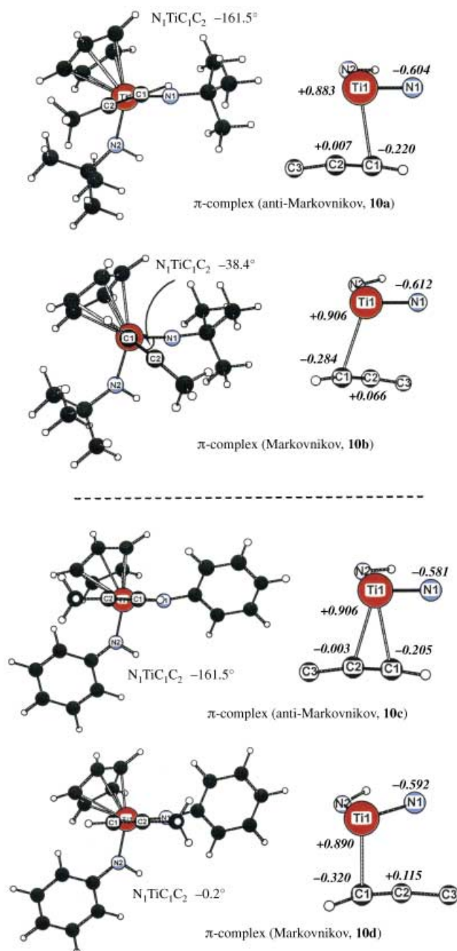
Figure 1. The computed N_1TiC_1C_2 torsion angles and natural charges (bold and italics) for the \pi -complexes of tert -butylamine (top) and aniline (bottom) as substrates.
