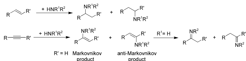
Scheme 1. Hydroamination of alkenes and alkynes.
