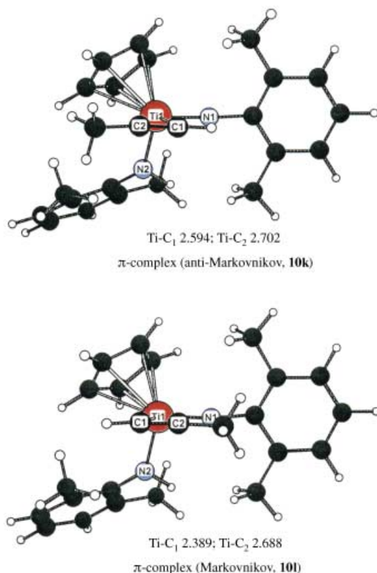
Figure 2. The conformation for the \pi -complexes of 2,6-dimethyl amine substrate [Å].
