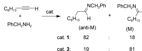
Scheme 3. Switch of regioselectivity.
