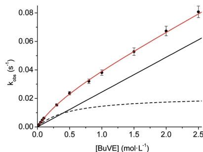
Figure 5. Fit of k_{\text{obs}} vs [\text{BuVE}] plot according to (eq 3, red curve) for complex 1 (H) displayed in the range [\text{BuVE}] = 0 - 2.55 \text{ mol}\cdot\text{L}^{-1} ( k_{\text{obs}} measured up to [\text{BuVE}] = 3.5 \text{ mol}\cdot\text{L}^{-1} ). The contribution of eq 2 (dashed line) and m_1 \cdot [\text{BuVE}] (solid line) is shown.
