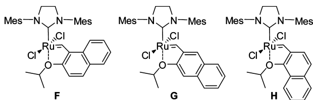
Scheme 2. Grubbs–Hoveyda-Type Complexes with Naphthyl Groups
