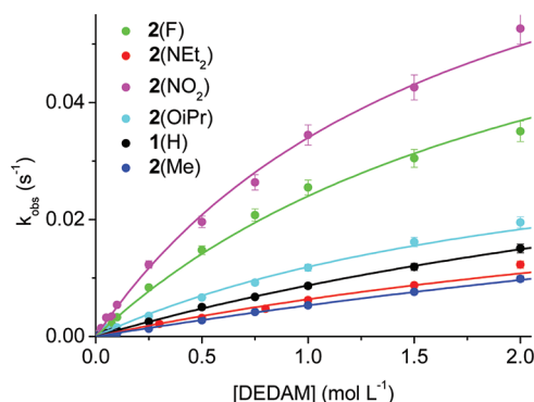
Figure 9. Plot of k_{\text{obs}} vs [DEDAM] for the five-substituted complexes 2.
