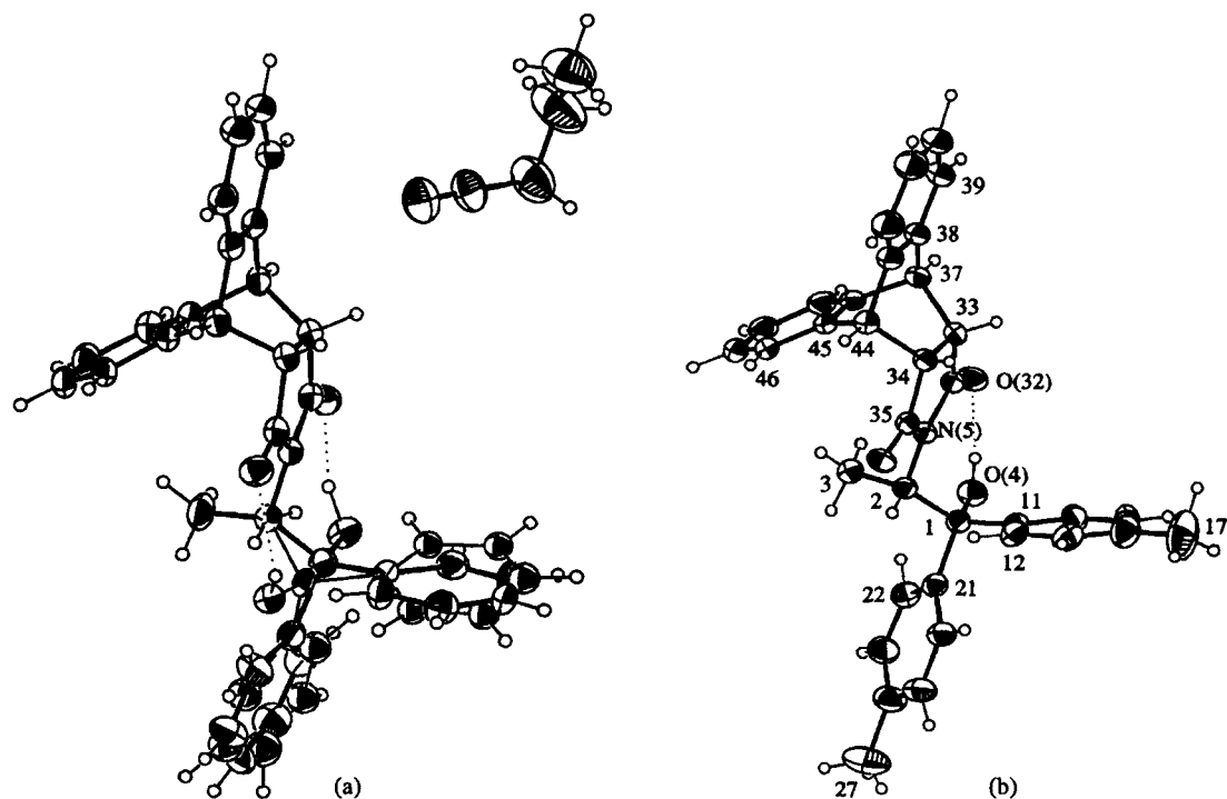
Figure 1. (a) An Ortep 37 view of the molecular structure of the 1b -butyronitrile complex showing the configurational disorder. The dotted line represents the intramolecular hydrogen bond. Ellipsoids are drawn at the 30% probability level. (b) Same for the optically resolved free host 2a
