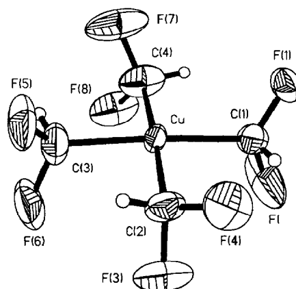
Fig. 4. A perspective drawing of the [\text{Cu}(\text{CF}_2\text{H})_4]^- anion in [\text{PNP}][\text{Cu}(\text{CF}_2\text{H})_4] with 20% probability thermal ellipsoids for the non-hydrogen atoms.
