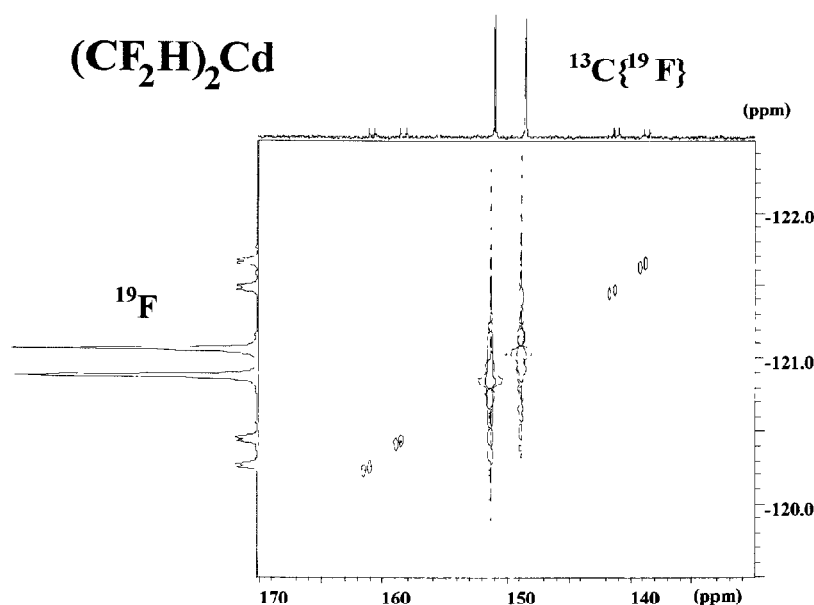
Fig. 2. 2D- ^{13}\text{C}/^{19}\text{F} -COSY spectrum of (\text{CF}_2\text{H})_2\text{Cd} . The signs of ^2J(\text{CdF}) and ^1J(\text{CdC}) as well those of ^1J(\text{CH}) and ^2J(\text{FH}) are equal.
