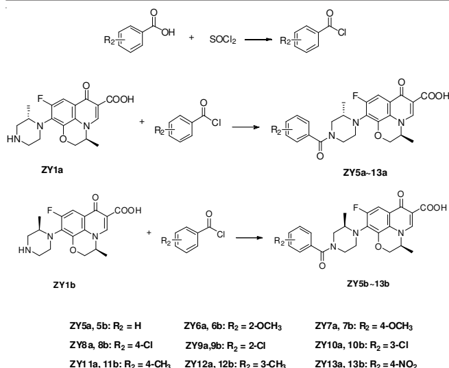
Scheme-IV: Synthetic routes to compounds ZY5a-13a and ZY5b-13b
