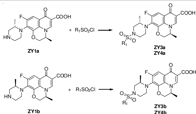
Scheme-III: Synthetic routes to compounds ZY3a , ZY4a , ZY3b and ZY4b
