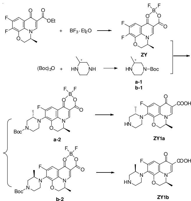
Scheme-I: Synthetic routes to compounds ZY1a and ZY1b
