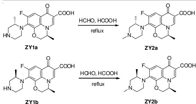
Scheme-II: Synthetic routes to compounds ZY2a and ZY2b
