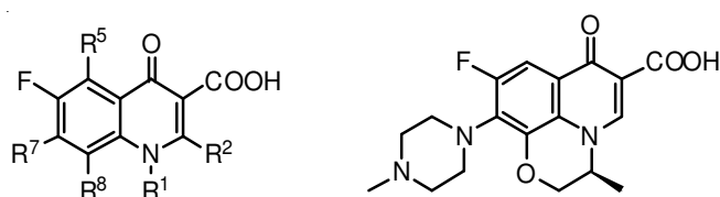
Fig. 1. Structural features of fluoroquinolones and levofloxacin
