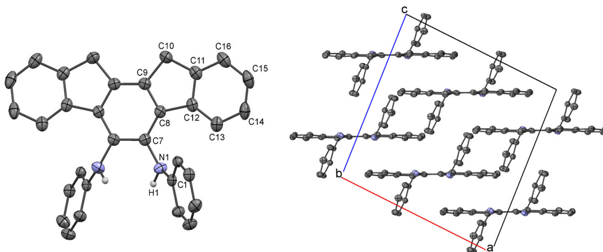
Figure 4. The molecular structure of [PhNH-C(C 6 H 4 )-C(C 6 H 4 )-NHPh] ( 2 ) and crystal packing. Hydrogen atoms on the indenyl and on the phenyl groups are omitted for clarity. The H attached at the N(1) and N(2) were localised in Fourier maps. Ellipsoids at 50% of probability.
