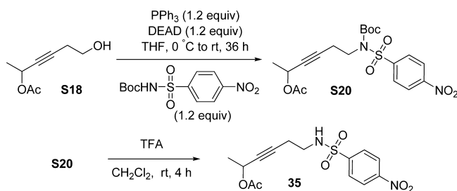
Scheme 15. Synthesis of Alkyne 35
