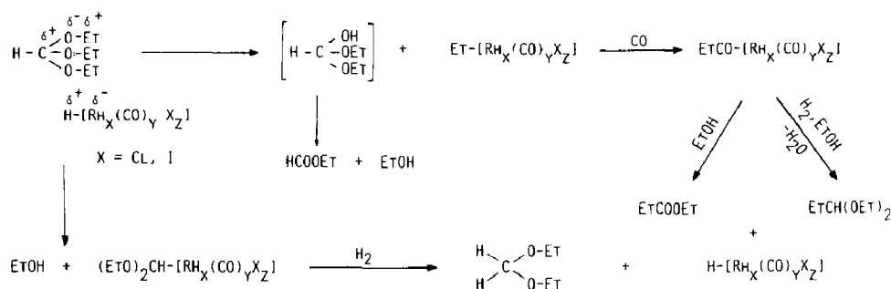
Scheme 4. Carbonylation and hydrocarbonylation of ethyl orthoformate in the presence of iodo- and chloro-carbonylrhodium derivatives.
