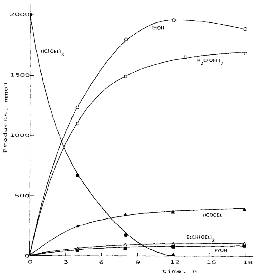
Fig. 2. Hydrocarbonylation of ethyl orthoformate in the presence of [\text{Rh}(\text{CO})_2\text{Cl}]_2 catalyst. [\text{Rh}(\text{CO})_2\text{Cl}]_2 : 1 mmol; \text{HC}(\text{OEt})_3 : 2 mol; T : 170^\circ\text{C} ; P : 8 MPa; \text{CO}/\text{H}_2 : 1.
