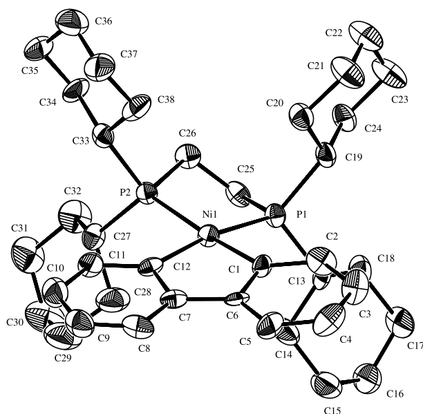
Fig. 1. Molecular structure of [\text{Ni}(2,2'\text{-C}_6\text{H}_4\text{C}_6\text{H}_4)(\text{dcpe})] ( 3 ) with selected atom labelling. Displacement ellipsoids show 30% probability levels; hydrogen atoms have been omitted for clarity.
