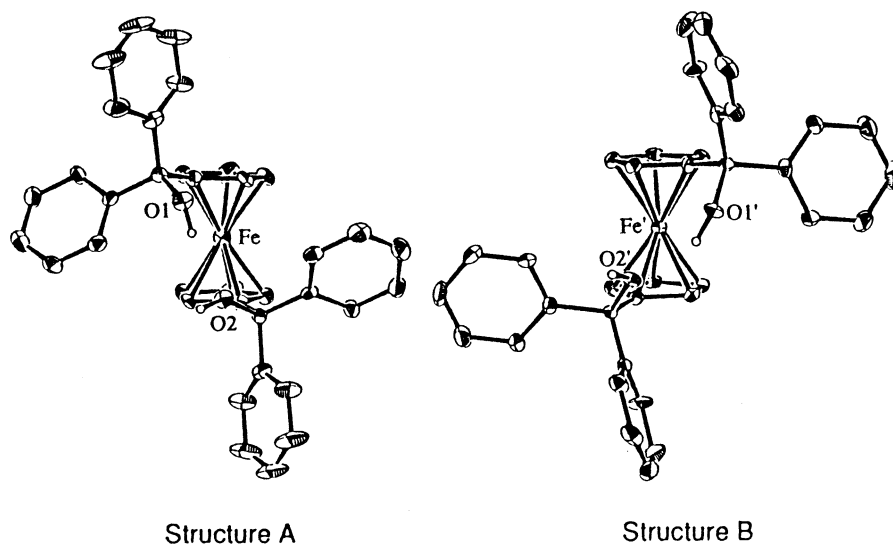
Fig. 1. Two crystal structures (A and B) of 5 (ORTEP, ellipsoids at the 20% probability level, R = 0.073 , R_w = 0.046 ).
