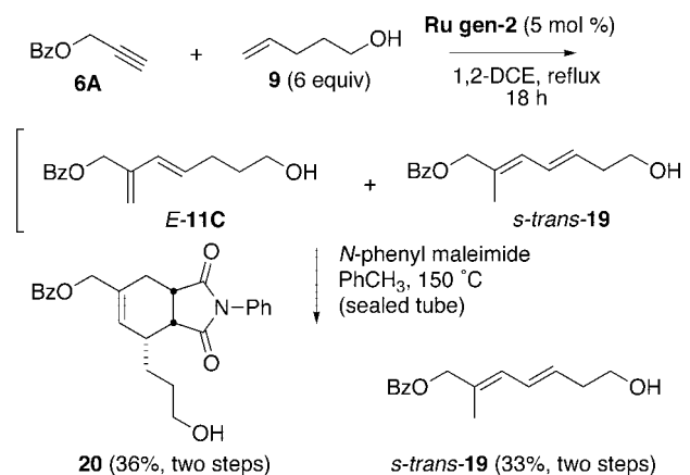
Scheme 3. Trapping of Isomerization Intermediate
