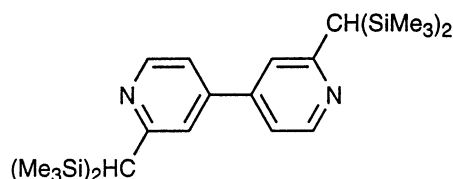
"Tail-to-tail" coupled alkyl
