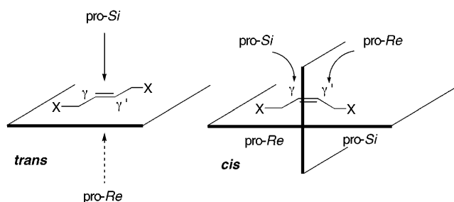
Scheme 8. Different enantiotopic faces for trans - and cis -1,4-dihalo-2-butenes.
