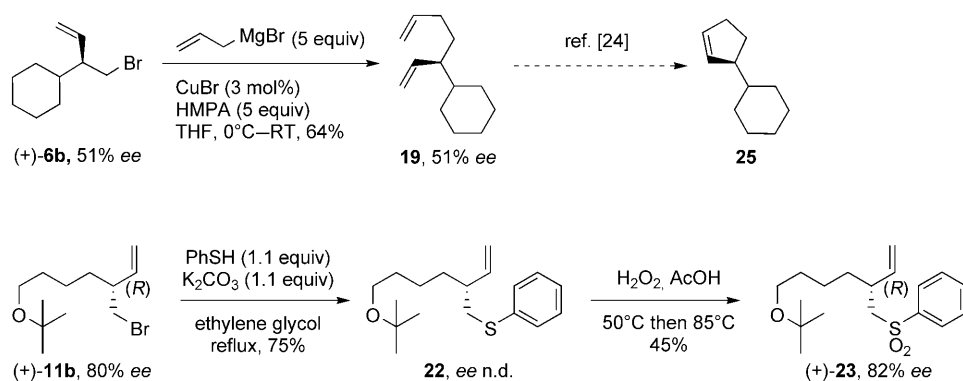
Scheme 15. Nucleophilic derivatization of chiral homoallylic bromides 6b and 11b .
