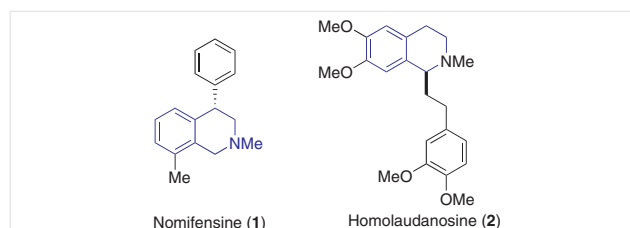
Figure 1 Structures containing isoquinoline alkaloids
