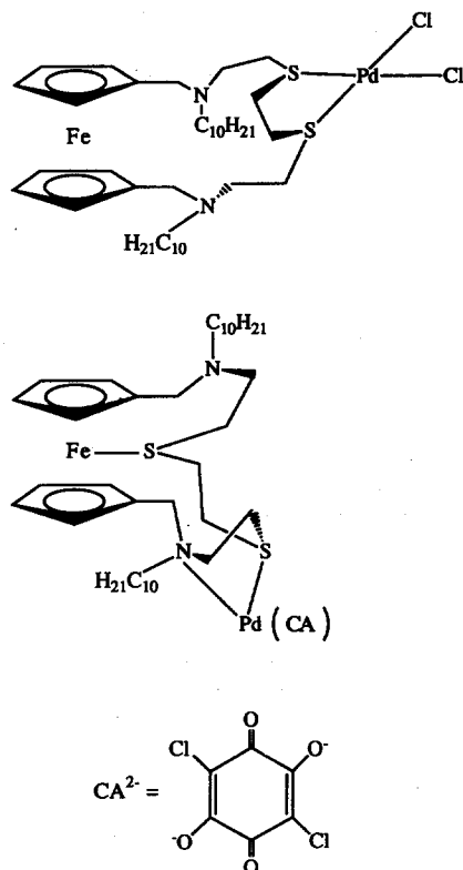
Fig. 1. Proposed structures of [\text{7}]\text{PdCl}_2 and [\text{7}]\text{Pd}(\text{CA}) .
