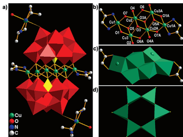
Figure 1. (a) Structure of polyoxoanion 1a . Color codes: WO 6 , red; SiO 4 , yellow. (b, c) Ball-and-stick and polyhedral representations of the Cu 6 hybrid unit in 1 , respectively. (d) Polyhedral representation of the Cu 6 unit in ref 9.
