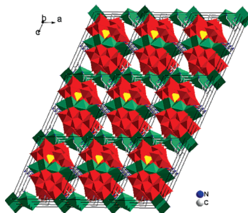
Figure 2. View of crystal packing of 1 along the b -axis. All the isolated water molecules and hydrogen atoms are omitted for clarity. Color codes: WO 6 , red; SiO 4 , yellow.
