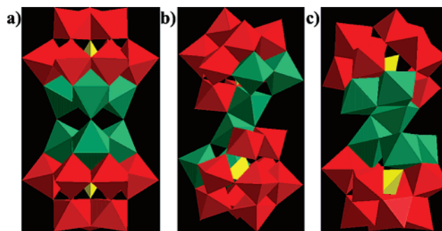
Figure 3. Polyhedral representations of (a) Fe 6 Ge 2 W 18 or Fe 6 Si 2 W 18 -1; (b) Fe 6 Si 2 W 18 -2; (c) Ni 6 Si 2 W 18 . Color codes: WO 6 , red; FeO 6 or NiO 6 , green; GeO 4 or SiO 4 , yellow.
