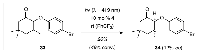
Scheme 8 Sensitized photocyclization of 2-(4-bromophenoxy)-3,5,5-trimethylcyclohex-2-enone ( 33 )
