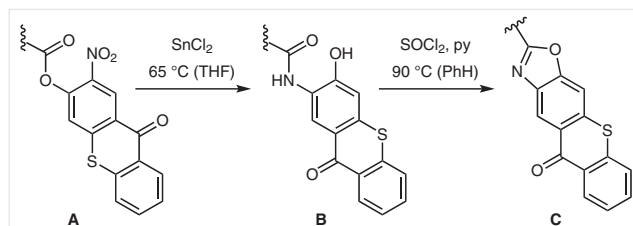
Scheme 2 Synthetic access to oxazole-annulated thioxanthones C starting with (2-nitrothioxanthone-3-yl) ester A
