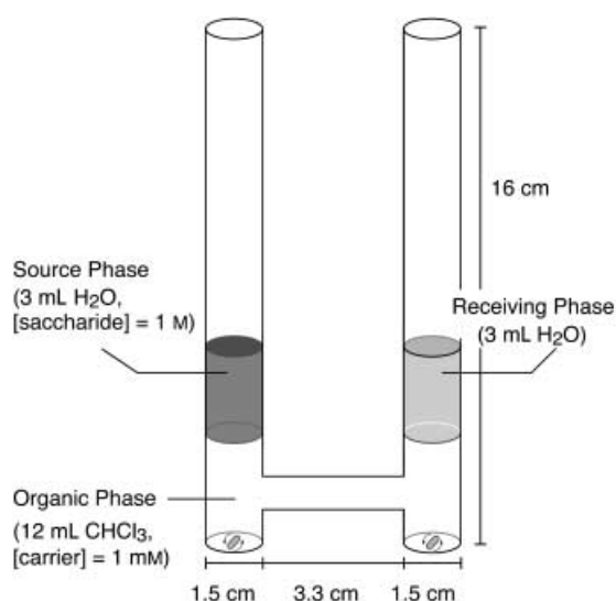
Figure 1. U-tube glass cell used for the transport experiments.
