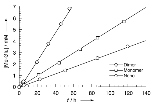
Figure 3. Time course of the concentration of methyl \alpha -D-glucopyranoside in the receiving phase. Source phase (3 mL \text{H}_2\text{O} , [\text{Me-Glu}] = 1.0 \text{ M} ); organic phase (12 mL \text{CHCl}_3 , [\textbf{1}] = [\textbf{2}] = 1.0 \text{ mM} ); receiving phase (3 mL \text{H}_2\text{O} ), 25 °C.
