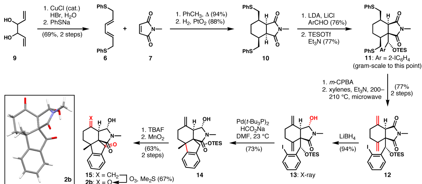
Scheme 2. Synthesis of the Tetracyclic “Core” of Exiguaquinol, Epimeric at C2
