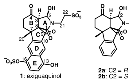
Figure 1. Exiguaquinol and tetracyclic model system hemiaminal diastereomers.
