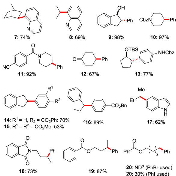
Figure 2. Coupling of aryl bromides with secondary alkyl bromides. (a) Reaction conditions: Ar-X (0.15 mmol, 100 mol %), PhBr (100 mol %), NiI 2 (10 mol %), 6c (10 mol %), Zn (200 mol %), MgCl 2 (100 mol %), pyridine (100 mol %), DMA (1 mL). (b) Isolated yields. (c) 1-Chloro-2,3-dihydro-1H-indene was used. (d) Not detected.
