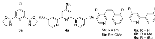
Figure 1. Structures of ligands.
