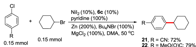
Scheme 1. Coupling of Activated Ar-Cl with Cyclohexyl Bromide a,b
