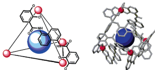
Figure 1. (Left) Schematic of M_4L_6 assembly with one of the edge-spanning ligands displayed containing a cartoon guest. (Right) Crystal structure of Fe_4L_6 assembly with a cartoon guest.
