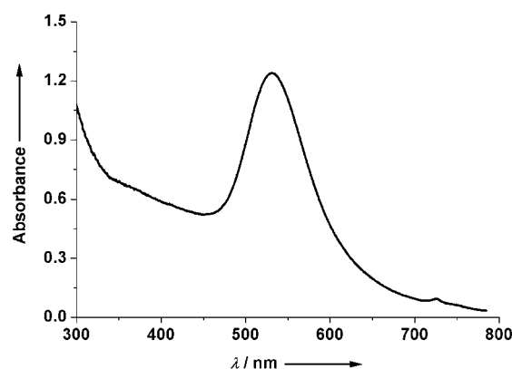
Figure 3. The UV-visible spectrum of Au nanoparticles in P104/ p -xylene/CO 2 /H 2 O microemulsion. P = 5.75 MPa, W_0 = 2.9 , [KBH_4] = [HAuCl_4] = 0.05 mol L -1 .
