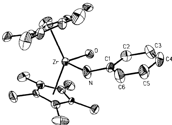
Fig. 2. Molecular structure of \text{Cp}_2\text{Zr}(\text{OH})(\text{NPh}) .
