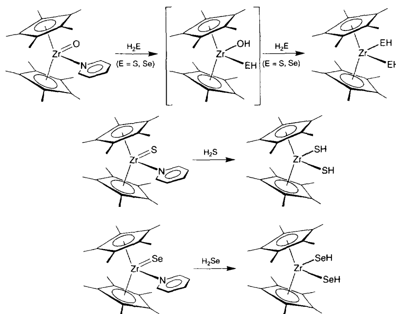
Scheme 5.
