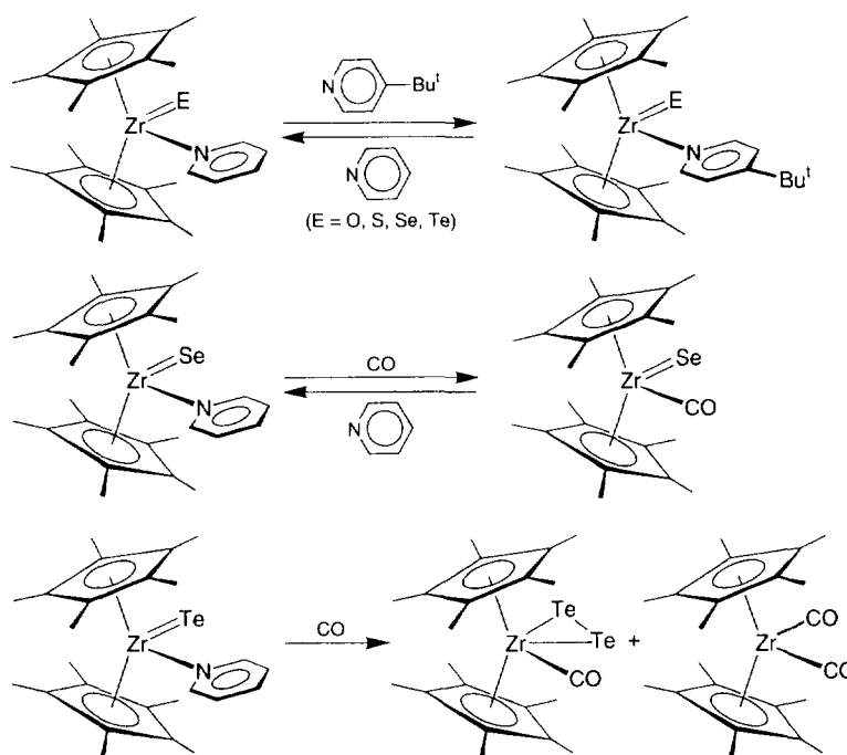
Scheme 13.
