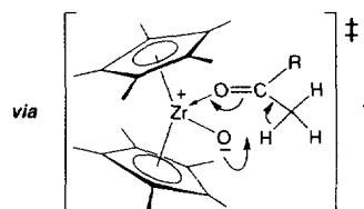
Scheme 9.
