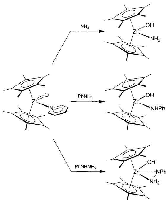
Scheme 7.
