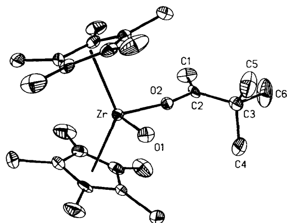
Fig. 3. Molecular structure of \text{Cp}_2^* \text{Zr}(\text{OH})[\eta^1\text{-OC}(\text{Bu}^t)=\text{CH}_2] .
