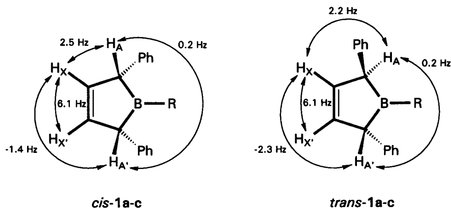
Fig. 1. Coupling constants J_{HH} for the 2,5-dihydro-1H-boroles 1a–1c.
