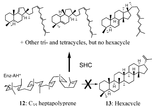
Scheme 2 Polycyclization products of heptapolyprenoid C 35 catalyzed by SHC. Large amounts of tri- and tetracyclic products are generated, but hexacyclic product 13 is not produced. 12
