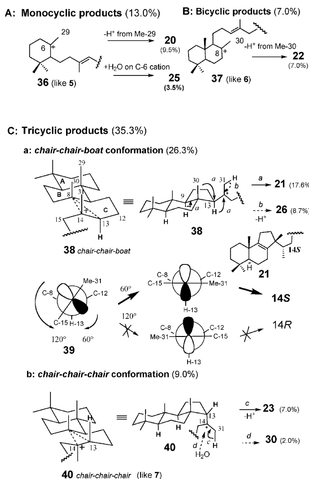
Scheme 5 Formation mechanisms of mono- (A), bi- (B) and tricyclic products (C).
