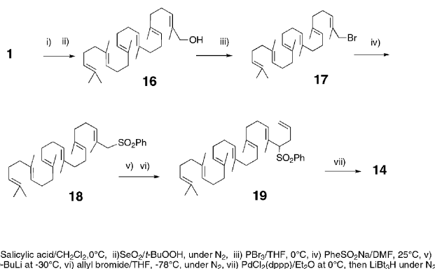
Scheme 4 Synthetic scheme of 14 .
