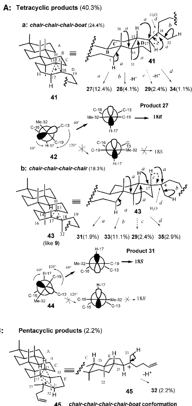
Scheme 6 Formation mechanisms of tetracyclic (A) and pentacyclic products (B).
